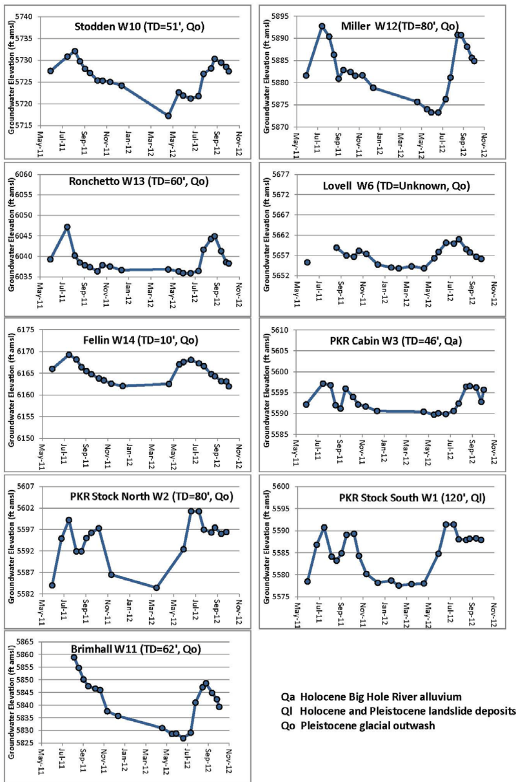
Figure 25: Wise River Hydrographs
